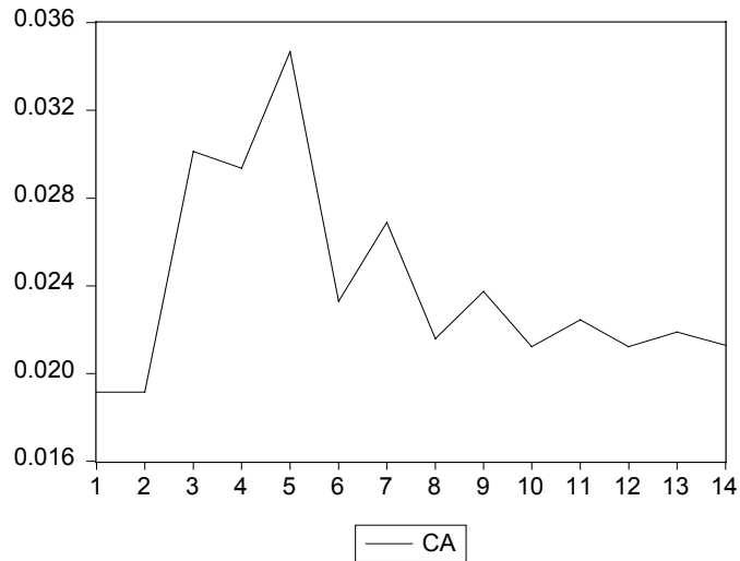
B. Simulated Equilibrium Path of Mexico's Current Account Deficit
