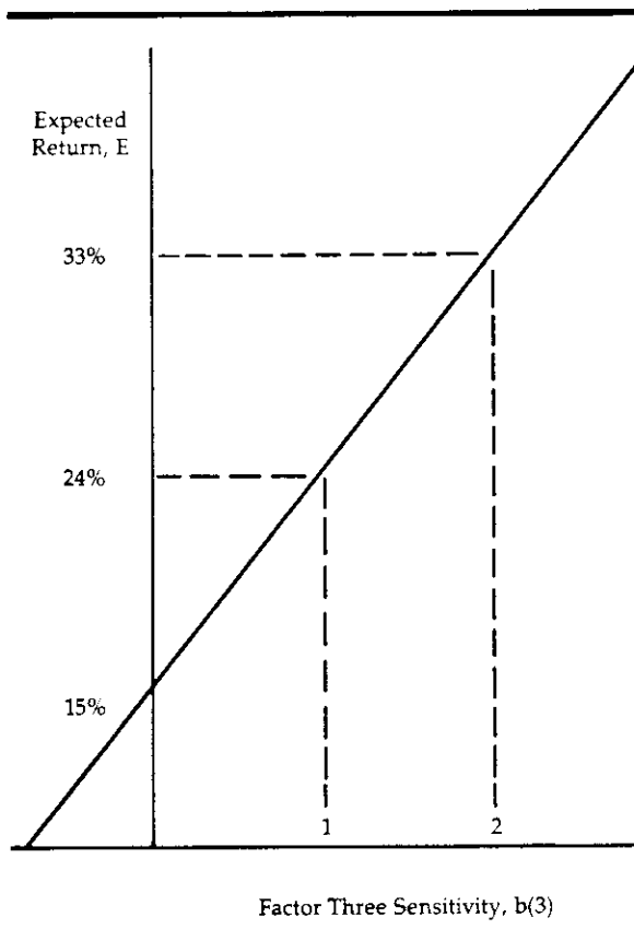
Figure D Equilibrium Expected Returns
