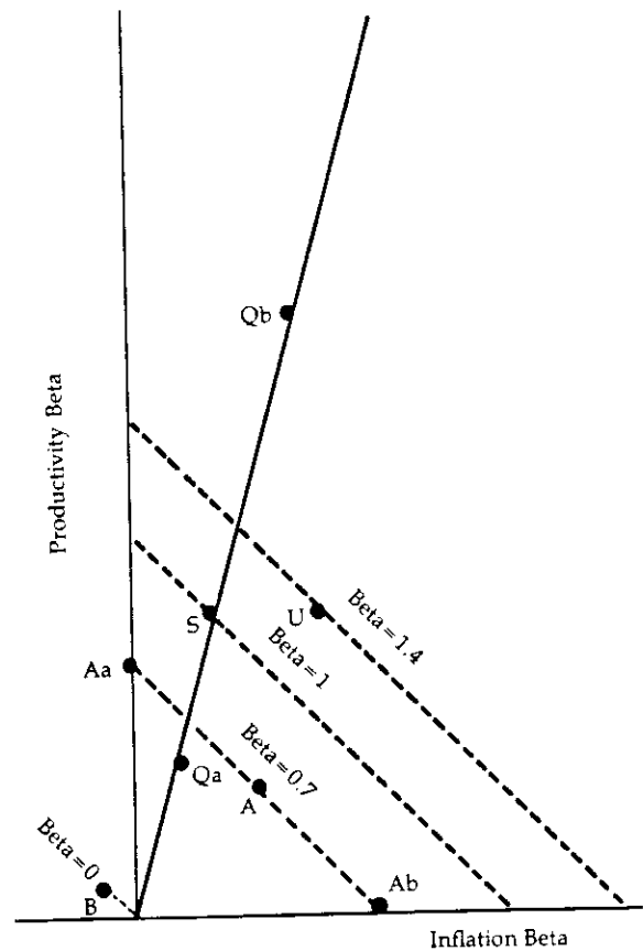
Figure F CAPM and APT Betas
